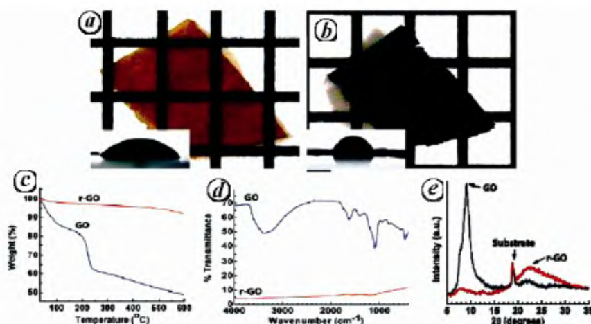
Figure 1. A GO paper (a) can be instantaneously reduced to r-GO (b) upon exposure to a photographic camera flash. The grids in the background are 1 mm × 1 mm. The flash reduction of GO to r-GO was evident by the dramatic changes in colour (a, b), water contact angle (insets), (c) TGA (d) FTIR and (e) XRD pattern. Reprinted with permission from Cote et al. 7 . Copyright (2009) from American Chemical Society.
